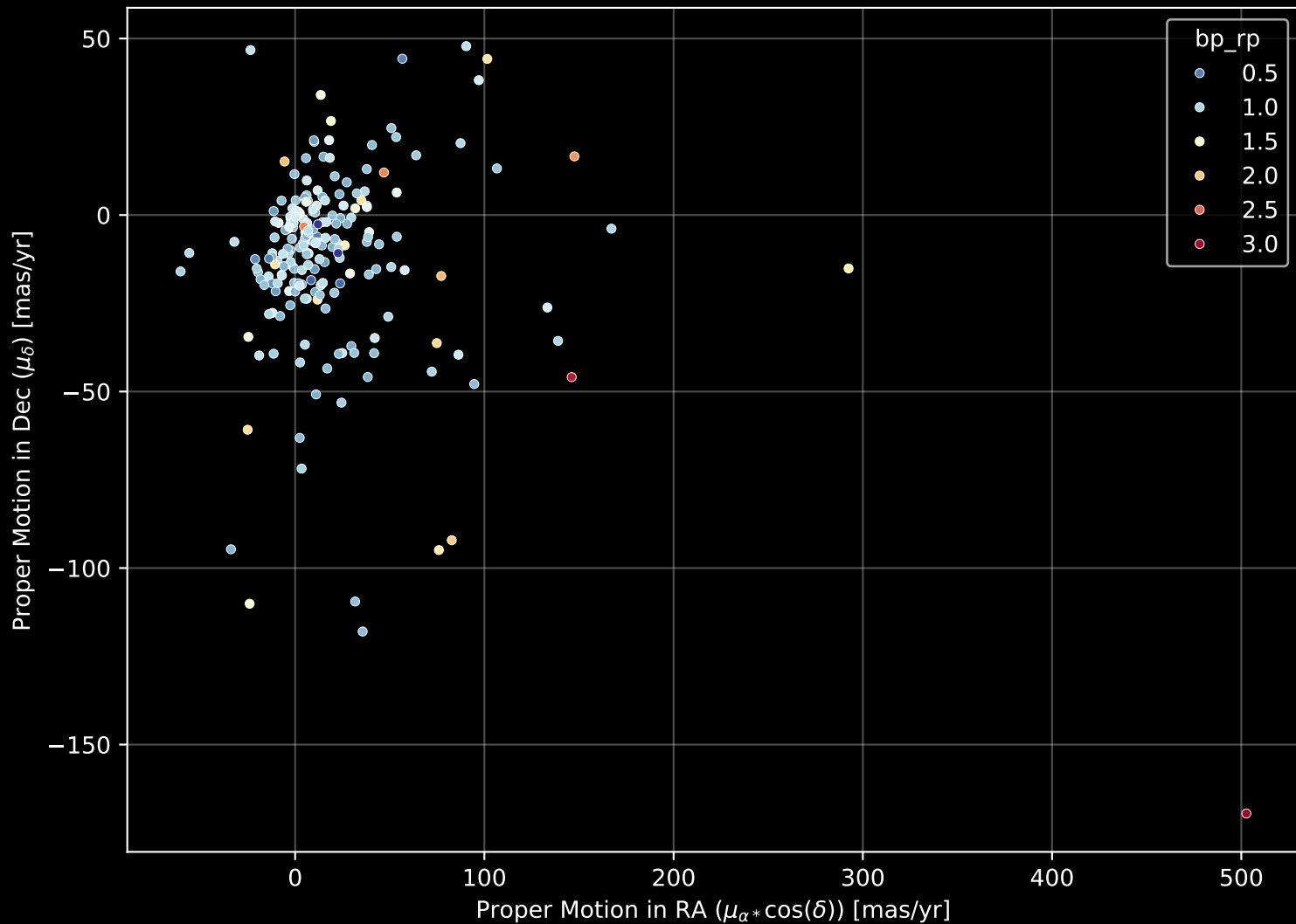
APOGEE DR17 Field: [169-54_MGA] Proper Motion Diagram (n = 207)
