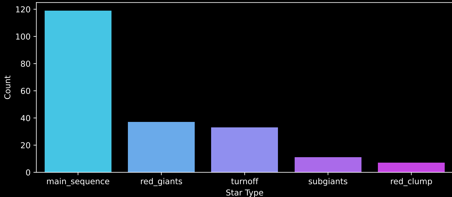
APOGEE DR17 Field: [169-54_MGA] Count plot of Star Type
