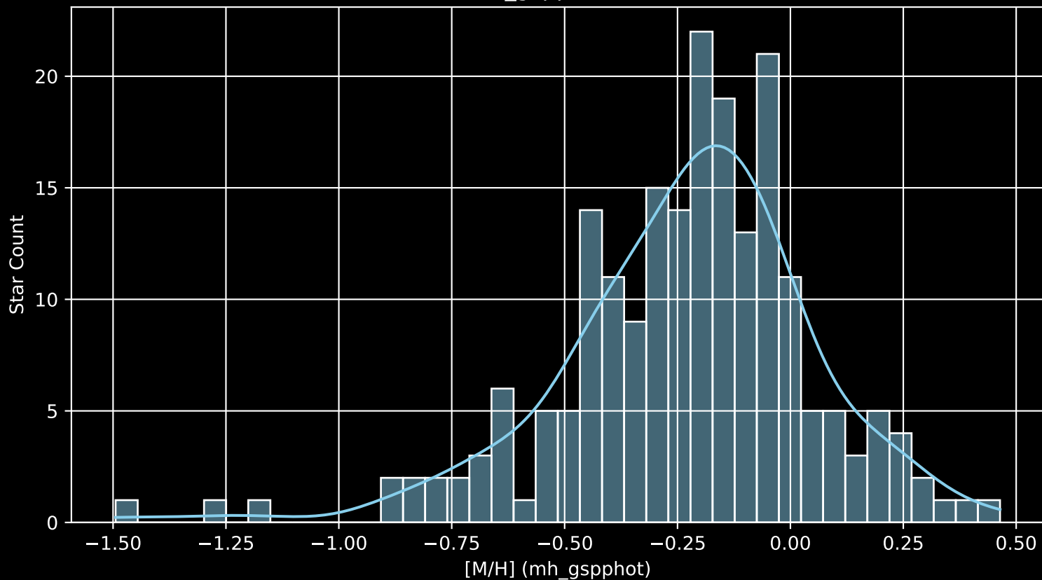
APOGEE DR17 Field: [169-54_MGA [M/H] (mh_gspphot) (n= 207)
