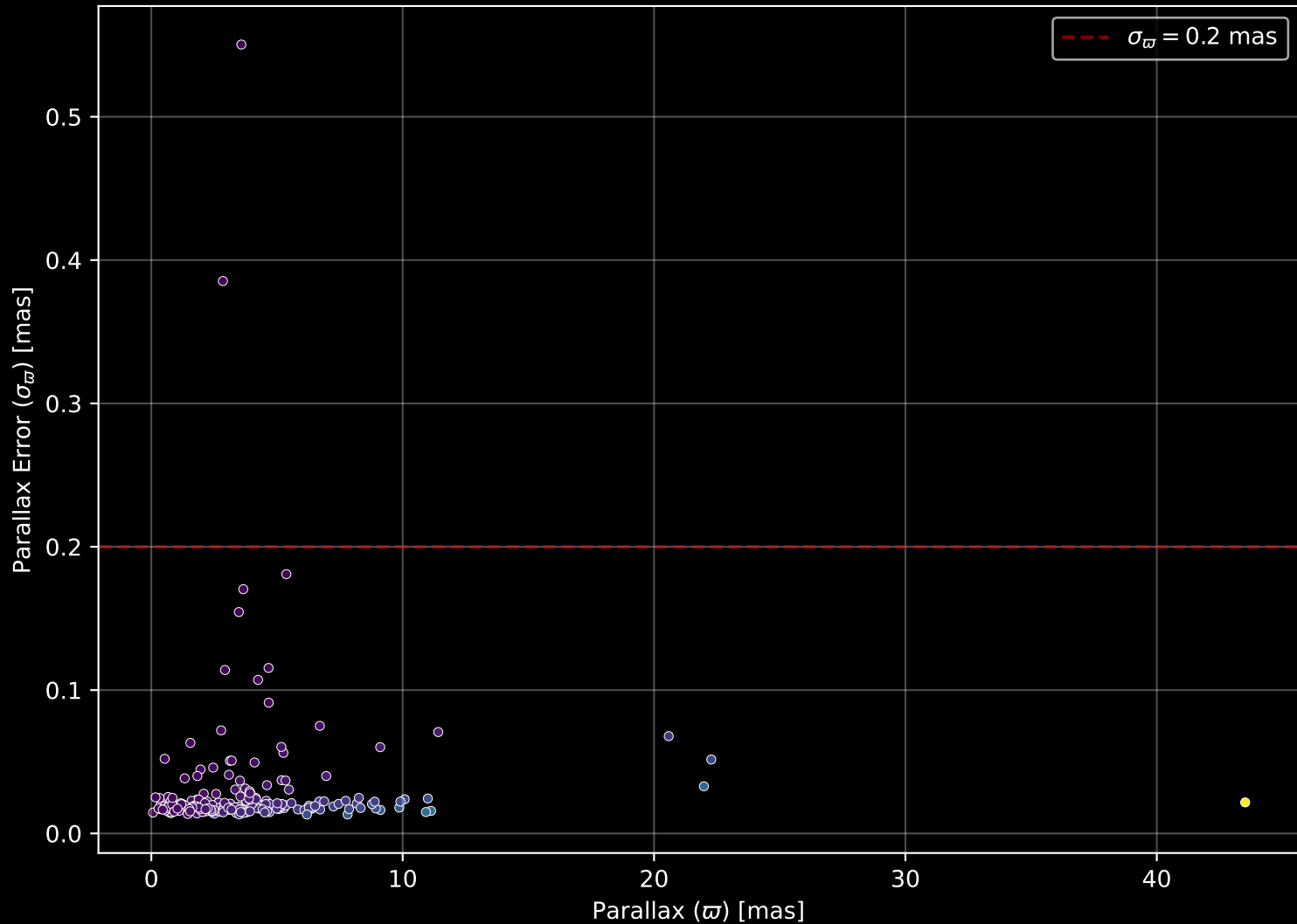
APOGEE DR17 Field: [169-54_MGA] Parallax Quality (n= 207)
