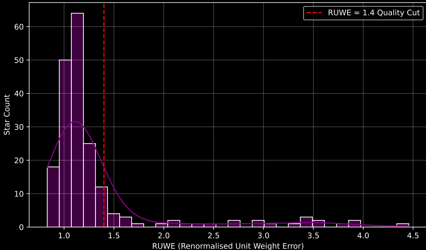
GAPOGEE DR17 Field [169-54_MGA] RUWE Distribution (n= 198)
