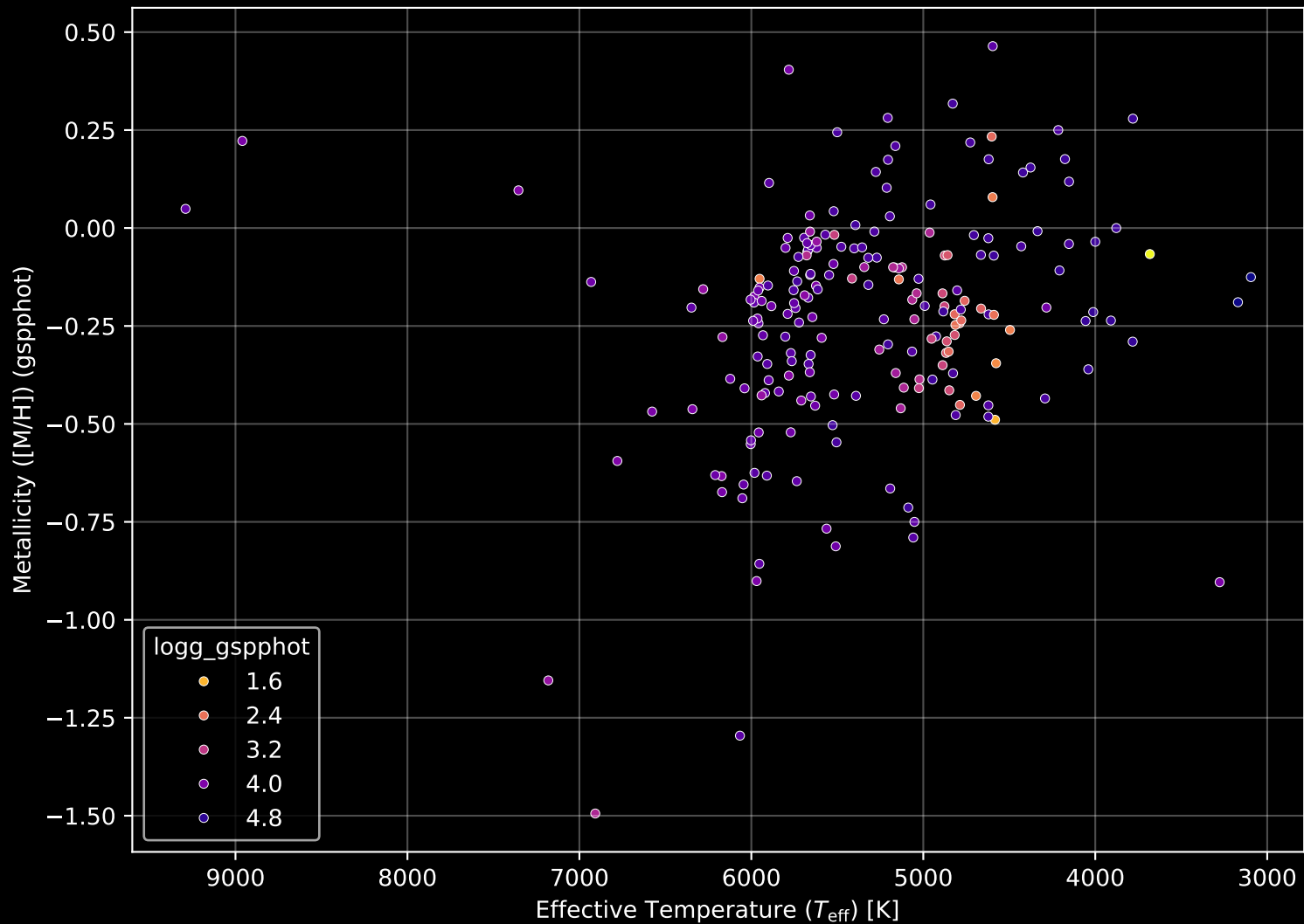
APOGEE DR17 Field: [169-54_MGA] Stellar Population Parameters (n= 207)
