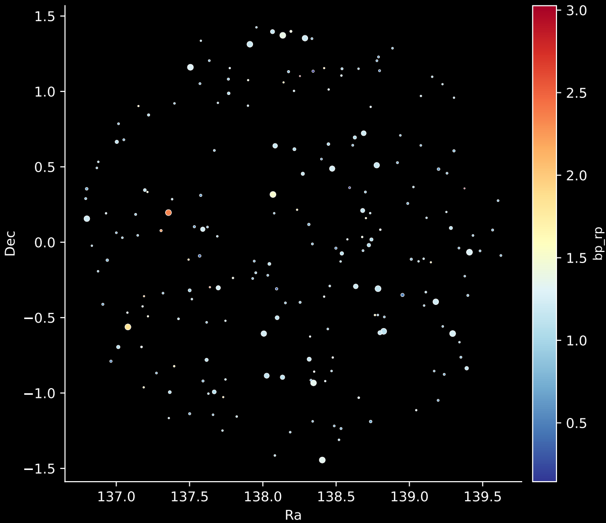
APOGEE DR17 Field: [169-54_MGA] Stars: 207
